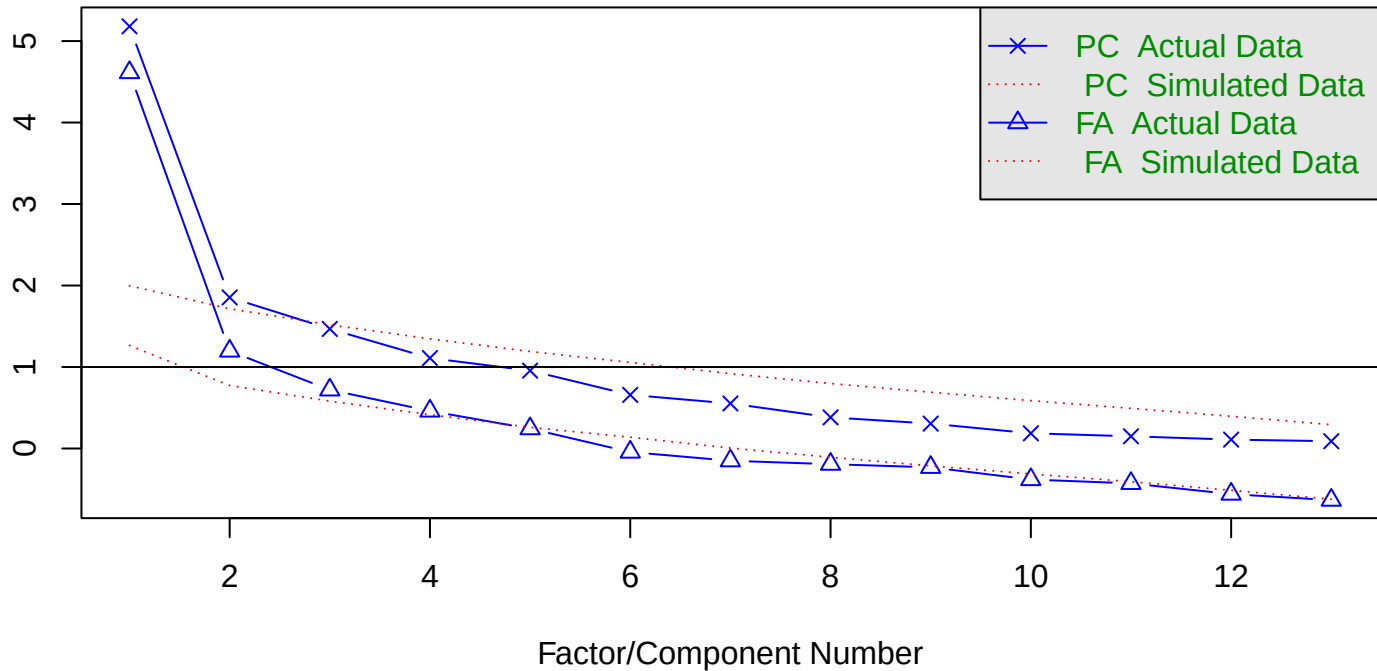
Parallel Analysis Scree Plot (MinRes) – Tableau
